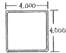
P330 POST 4" X 4" X .125" EXTRUDED ALUMINUM
